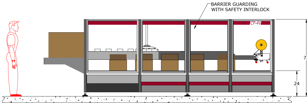
SIDE VIEW
